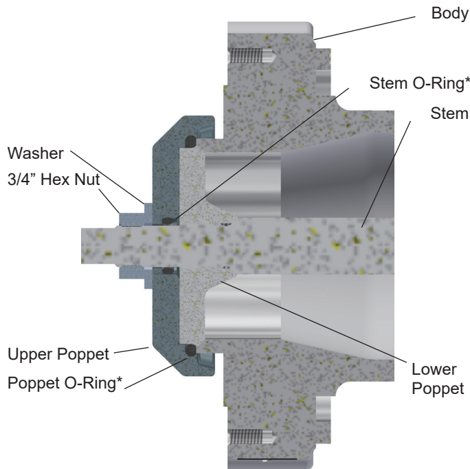
A8890S Series
