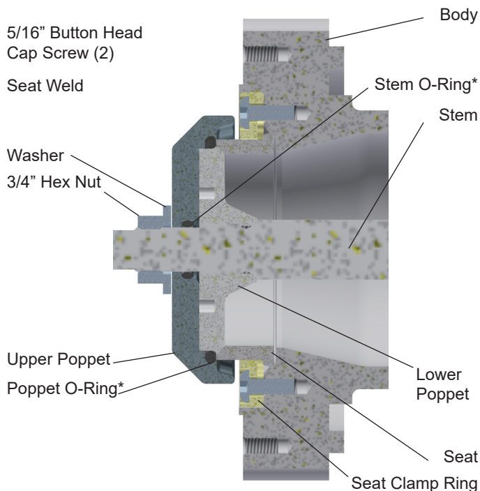
A8890W Series
