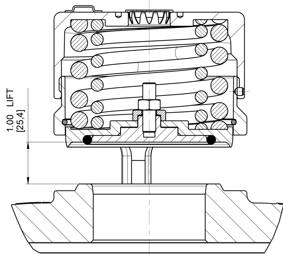
VALVE IN OPEN POSITION SECTION A-A SCALE 3:4
